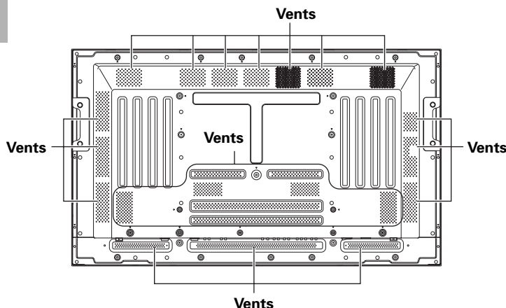
Illustration depicts PDP-5004 model.
