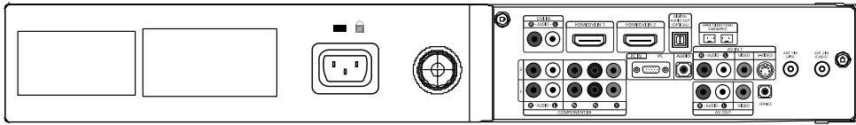
JACK PANEL DETAIL 3.25" H x 9.92" W @ 12.98" UP FROM BOTTOM
