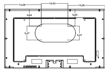
D-BOX MOUNTING HOLES FOR MODEL M4210C-BA
