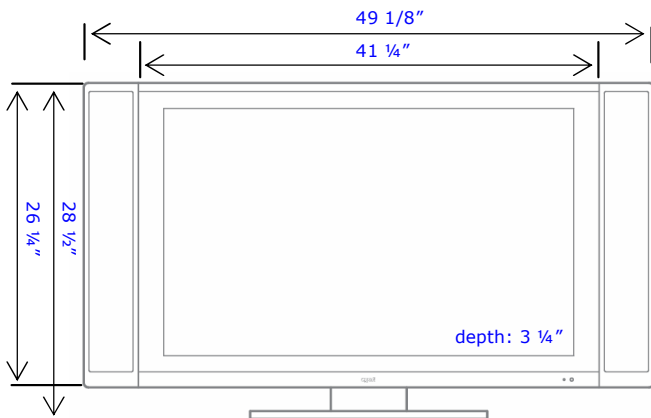
product dimensions
