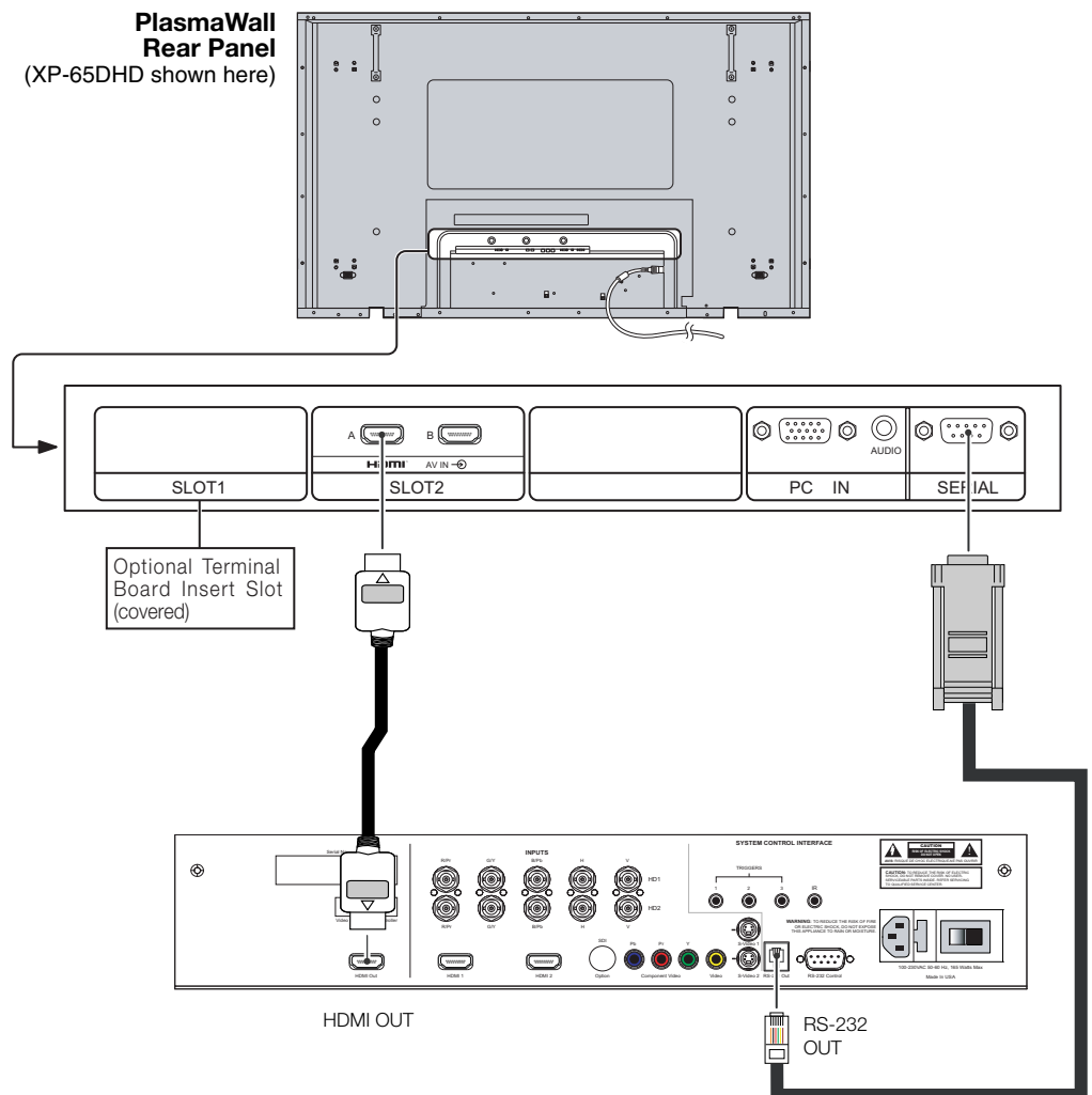
Figure 3-4. Connecting the PlasmaWall to the DHD Controller
