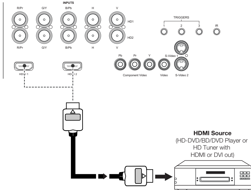
Figure 3-6. HDMI Source Connections
