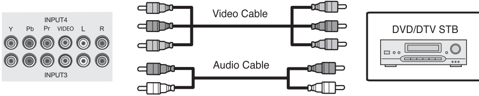
Figure 3-4. Component Video Connections
