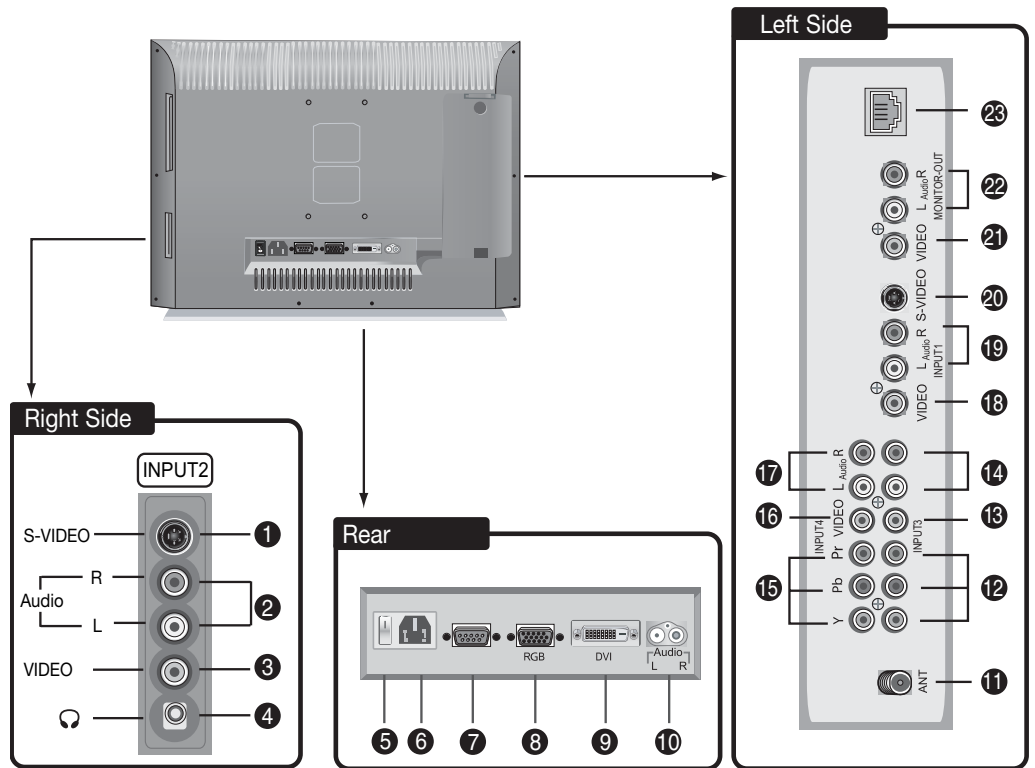
Figure 2-2. DView Connectors
