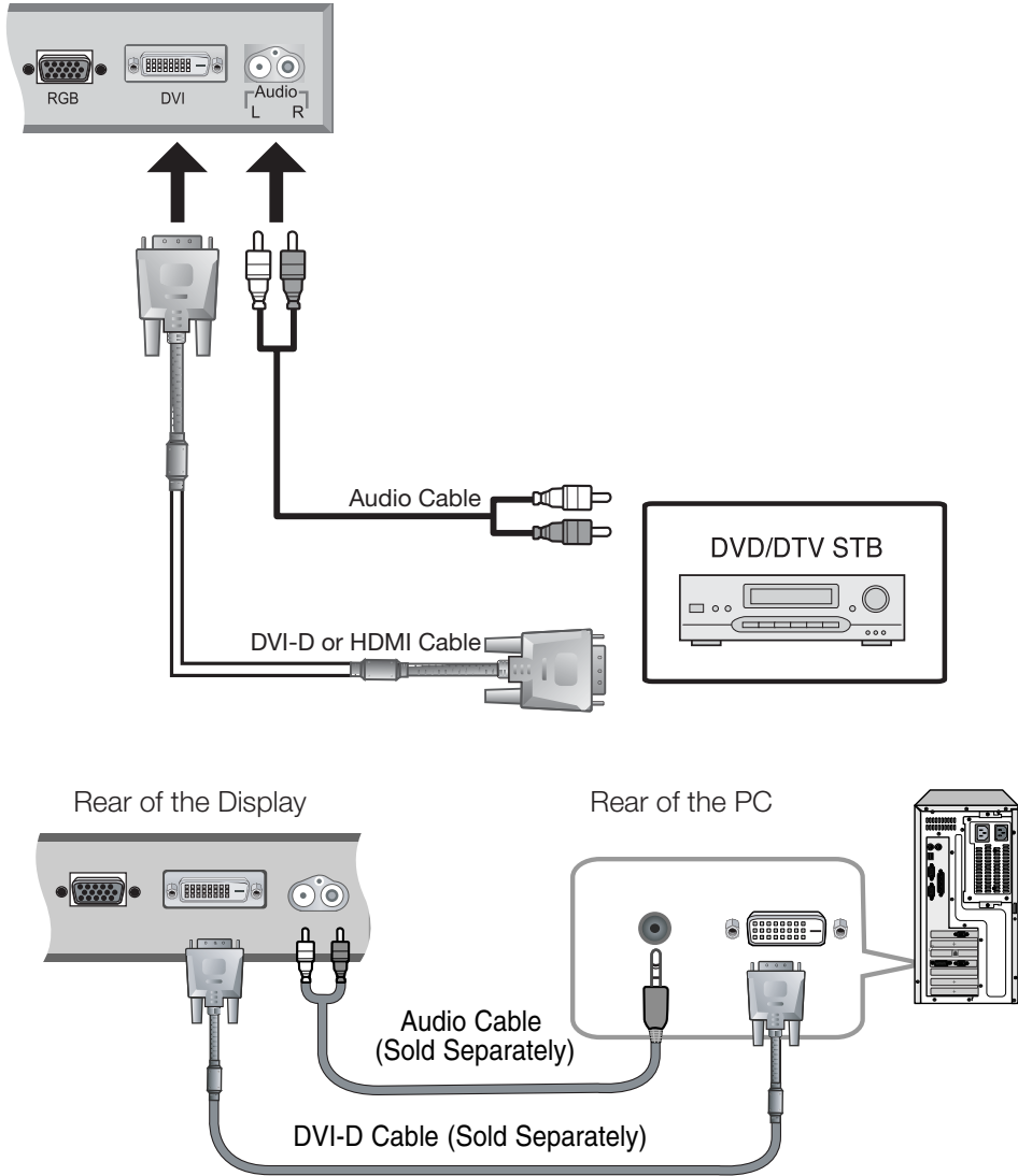
Figure 3-2. DVI or HDMI Source Connections
